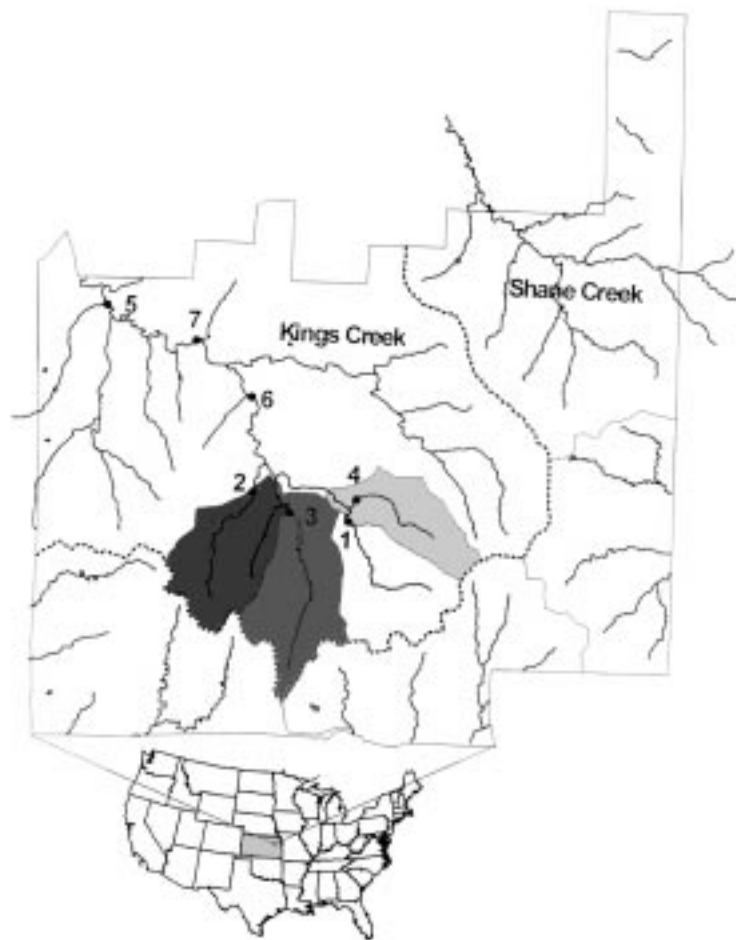
Figure 1. Watersheds and sampling locations used in this study. Numbers correspond to sample site numbers in Table 1. Sites 1, 2, 3 and 4 are found in the smallest individual watershed units nested within successively larger watershed units (Sites 5, 6 and 7). North is at the top of the map and from the east to west boundaries of Konza is 6.75 kilometers.
