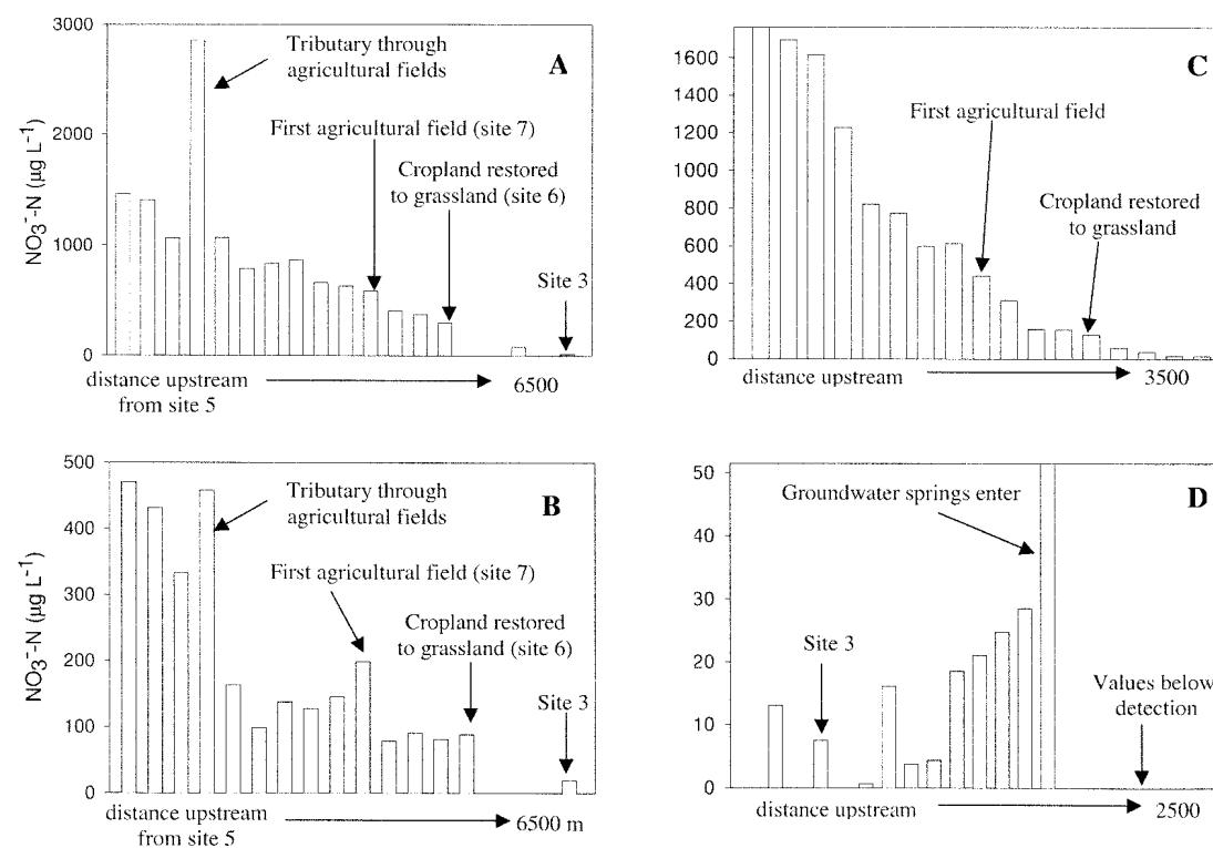
Figure 4. Temporal and spatial variations in \text{NO}_3^- concentrations on linear stream transects. Lower Kings Creek watershed in summer 1995 (A) and in winter 1998 (B). Shane Creek watershed in summer 1995 (C) and Upper Kings Creek watershed in summer 1995 (D). Data in Graph A were previously published in Gray et al., 1998.
