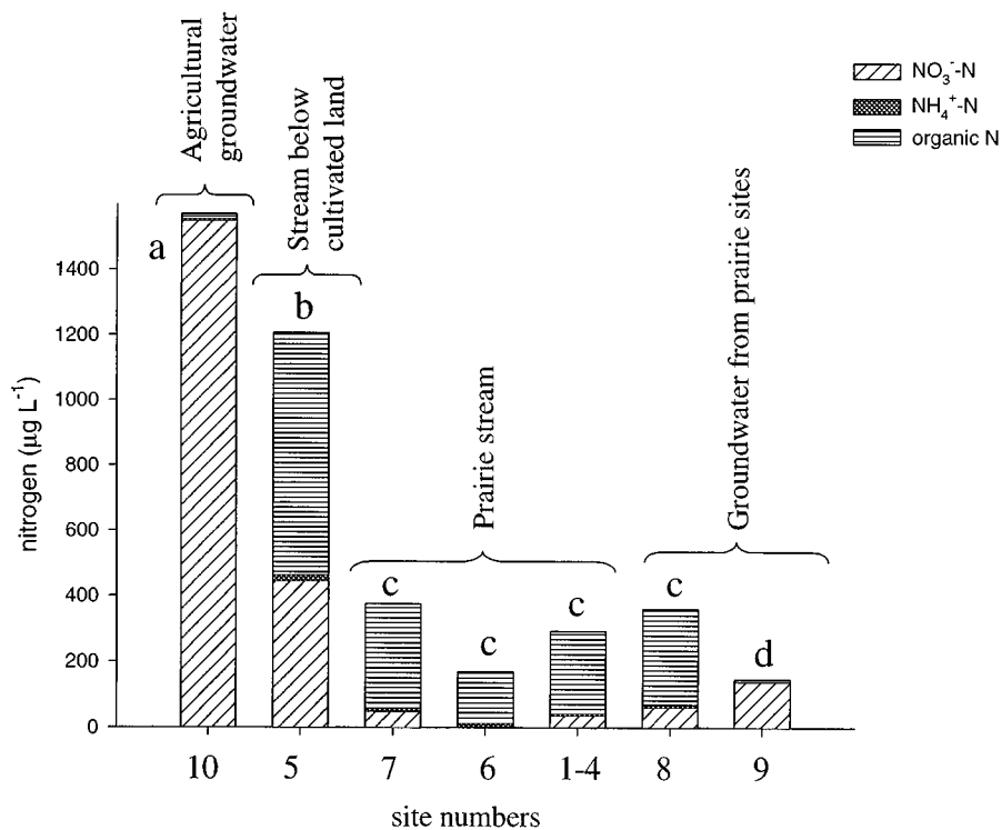
Figure 3. Nitrogen components of surface and groundwater within the Kings Creek watershed. Bars with different letters indicate sites that had significantly different \text{NO}_3^- concentrations ( \alpha = 0.05 , Student-Newman-Keuls multiple comparison, overall ANOVA was significant at p < 0.0001 ). Numbers for each bar correspond to sample site numbers in Table 1. n ranged from 36 to 543 per bar.
