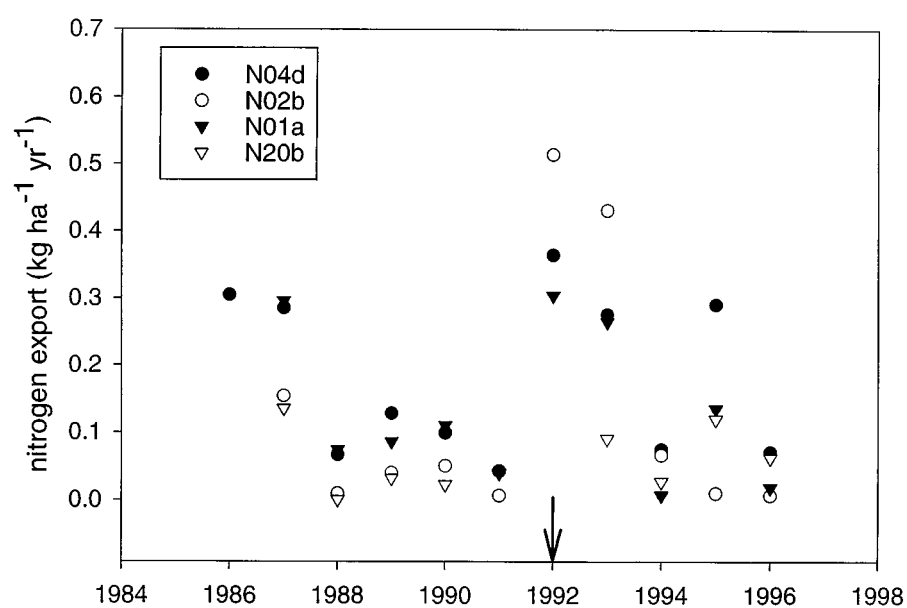
Figure 7. Nitrogen export over time for four watersheds. Arrow indicates the year in which bison were introduced onto the watersheds. See Table 1 for description of sites.
