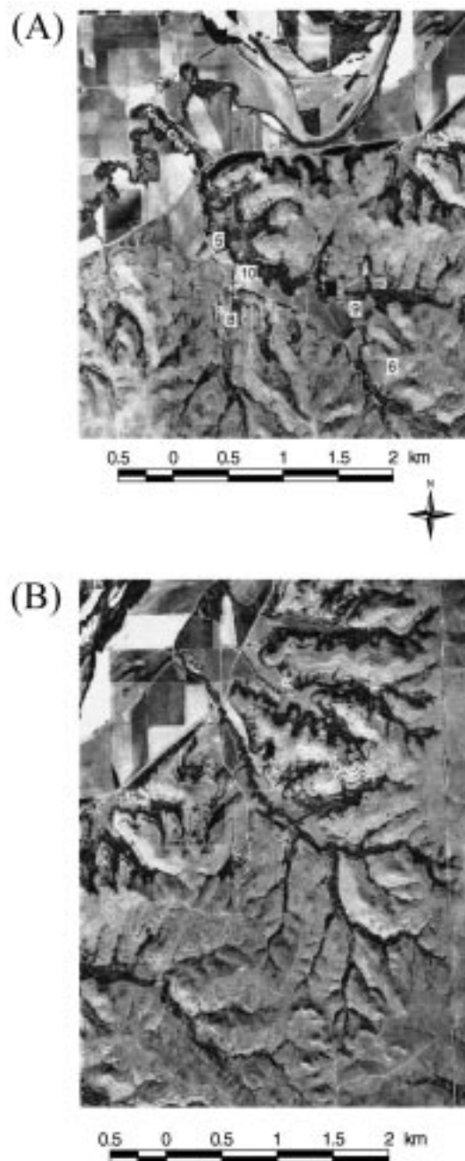
Figure 2. Aerial photographs of the lower reaches of Kings Creek (A) and Shane Creek (B) watersheds. Extensive riparian vegetation (gallery forest) occurs throughout the lower portions of both watersheds. Fertilized cropland occurs to the southwest of the stream channel between sites 7 and 5 in Kings Creek. Numbers correspond to sample site numbers in Table 1. Fertilized cropland in Shane Creek occurs on both sides of the stream channel downstream from the uppermost dirt road that crosses the channel.
