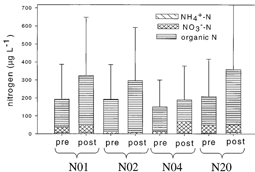
Figure 6. Total N, \text{NH}_4^+ , \text{NO}_3^- , and organic N concentrations at four sites before and after the introduction of bison. Error bars = 1 standard error of TN concentration.
