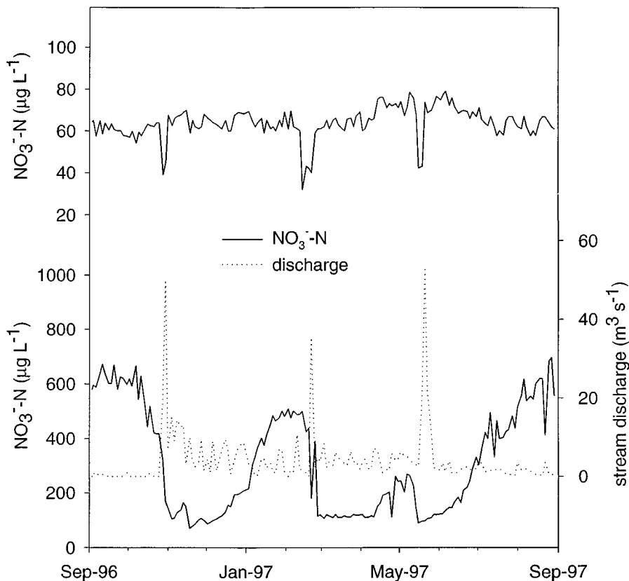
Figure 5. Changes in \text{NO}_3^- concentration and stream discharge over time. Groundwater from under prairie (site 9) is the top solid line and surface water below row-crop agriculture is the bottom solid line (site 5).
